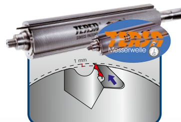
TERSA-HOBELMESSERWELLE
